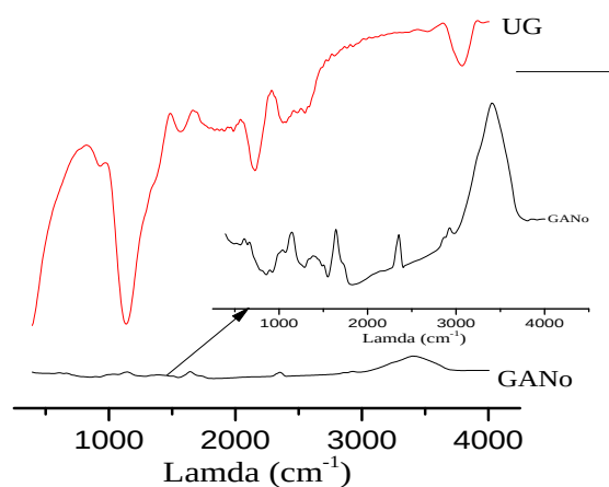
Figure 3- FTIR spectra of the unmodified modified kenaf shive sorbent
