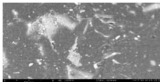
Fig. 6: SEM image of CP/HDPE composite B at 40% filler loading without coupling agent
