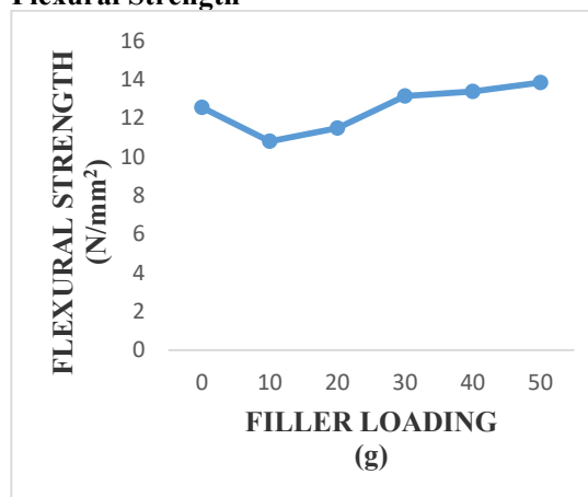
Figure 8: Effect of Nano Silica the Flexural Strength of the Composite
