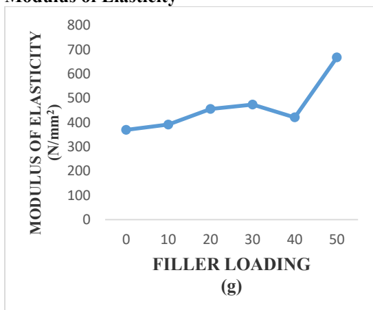
Figure 9: Effect of Nano Silica the Modulus of elasticity of the Composite
