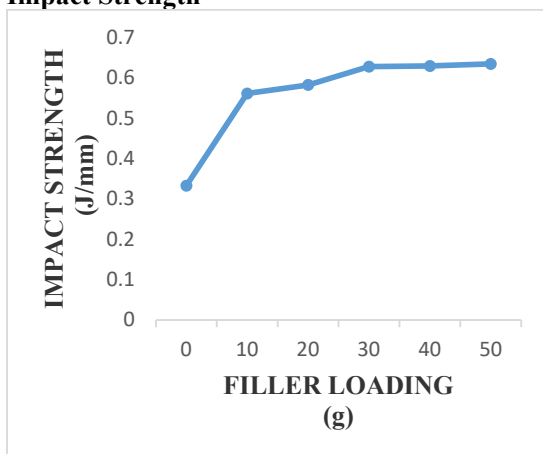
Figure 7: Effect of Nano Silica the Impact Strength of the Composite
