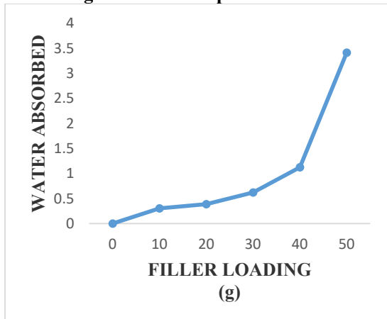
Figure 3: Effect of Nano Silica on the Water Absorption of the composite
