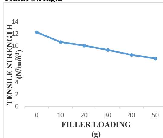
Figure 4: Effect of Nano Silica on the Tensile Strength of the Composite
