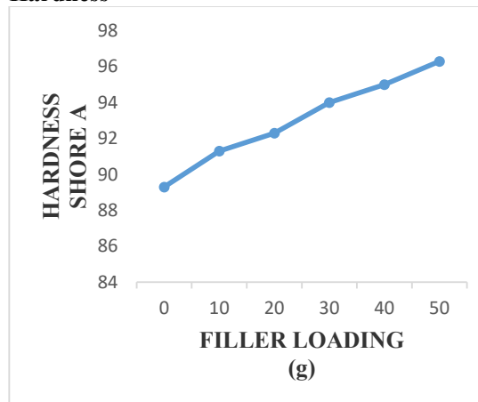
Figure 6: Effect of Nano silica on the Hardness property of the composite
