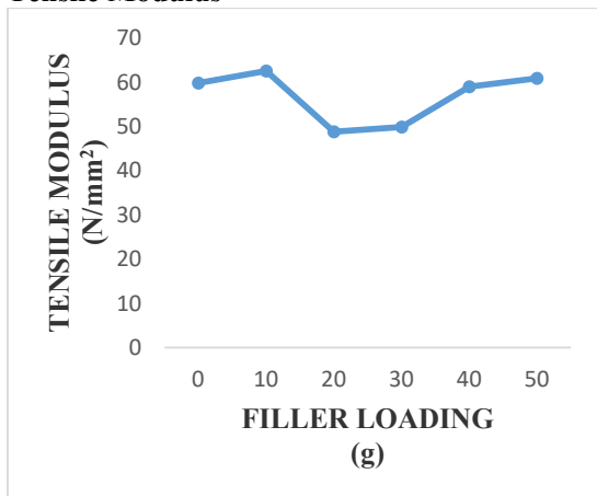
Figure 5: Effect of Nano Silica on the Tensile Modulus of the Composite
