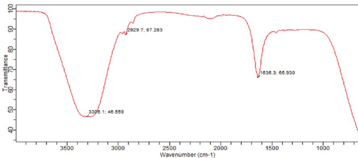
Fig. 5 FTIR Spectrum of Sea Water Offshore.
