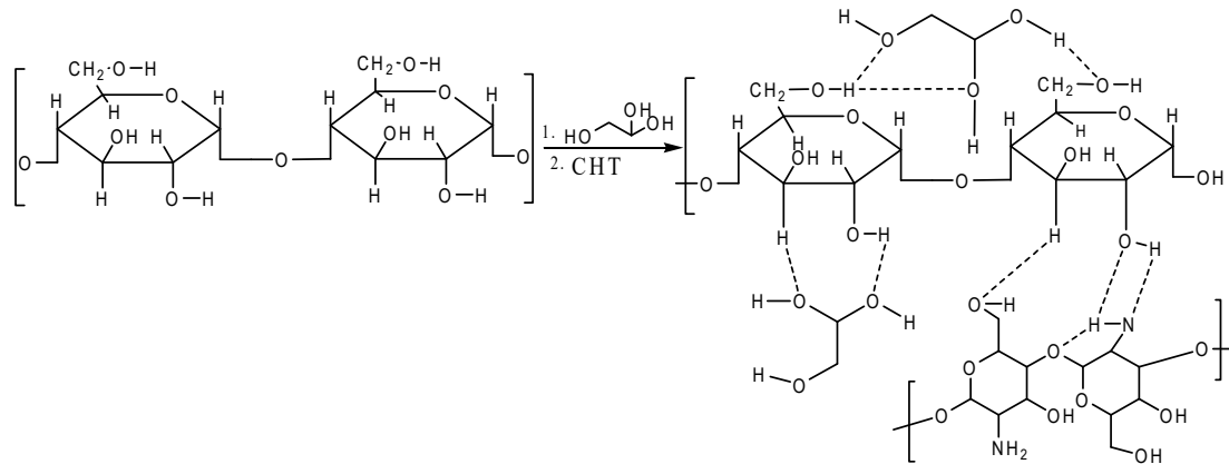
Scheme 1: Proposed molecular interaction between starch and glycerol (Enrique et al. , 2021).
