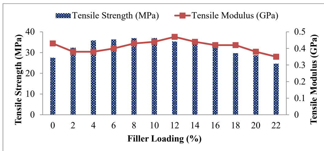
Figure 1. Effect of Filler Loading on Tensile Strength and Modulus of UP-FSP Composites
