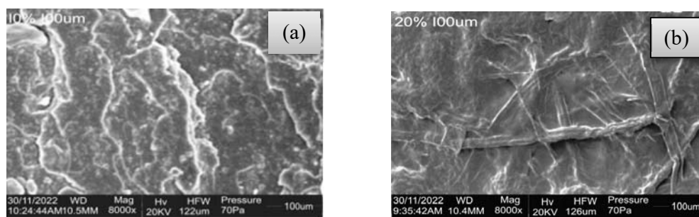
Figure 4: SEM Micrographs of fractured surface of UP-FSP Composites (a) 10 wt % and (b) 20 wt % filler loadings at a magnification of 8000X.
