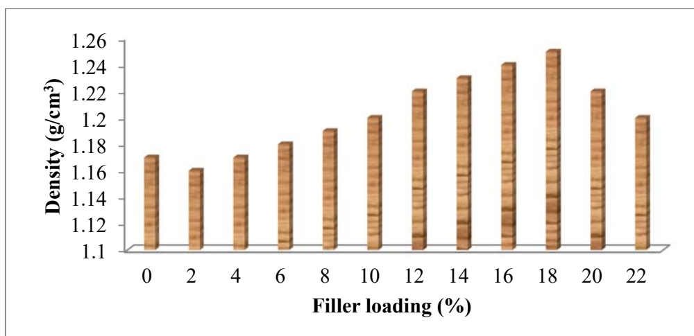
Figure 3. Effect of Filler Loading on Density of UP-FSP Composites
