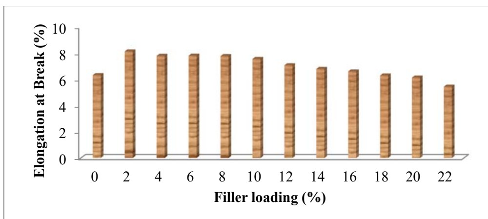
Figure 2. Effect of Filler Loading on % Elongation at Break of UP-FSP Composites
