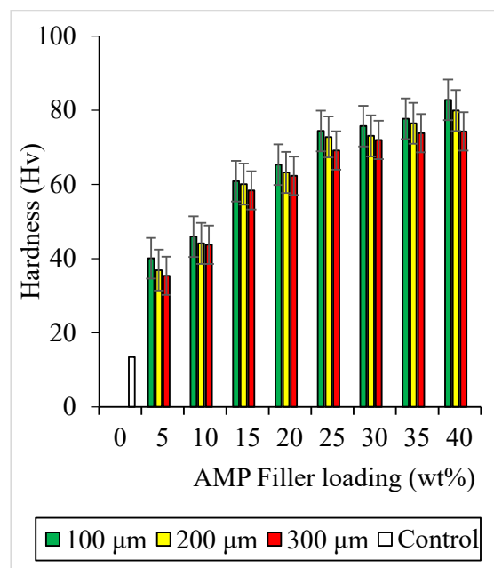
Figure 6: Effect of filler loading and particle size on the hardness of AMP/ER composite
