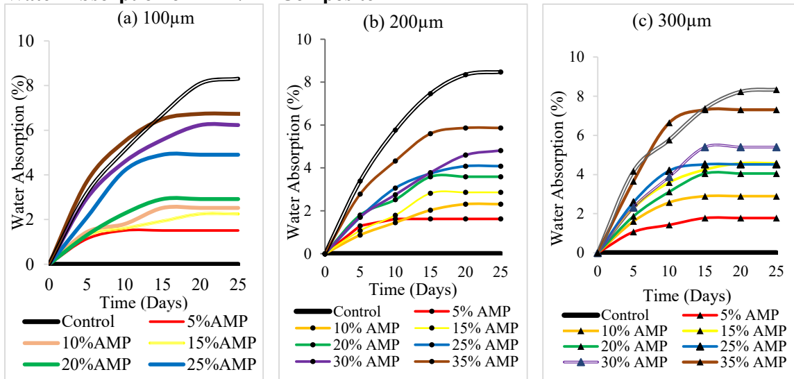
Figure 2(a-c): Effect of filler loading and particle size on water absorption of AMP/ER composites
