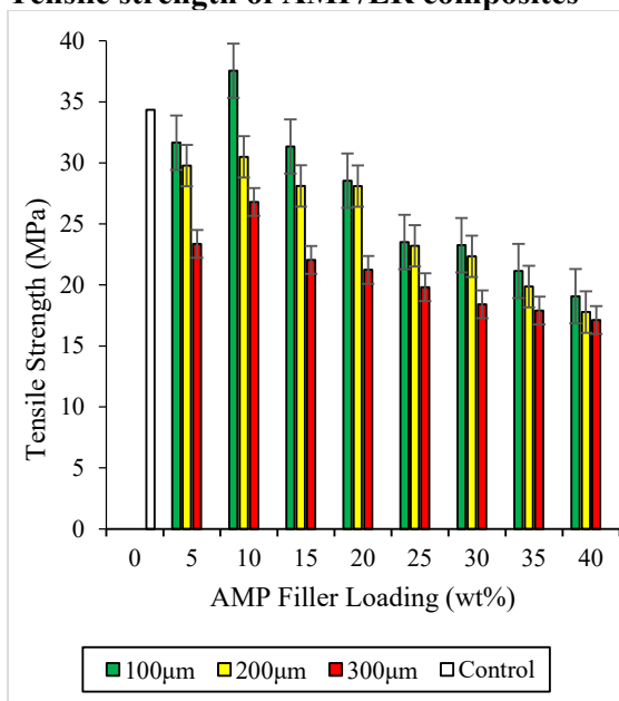
Figure 3: Effect of filler loading and particle size on tensile strength of AMP/ER composites
