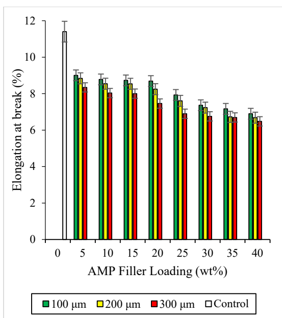
Figure 5: Effect of filler loading and particle size on elongation at break of AMP/ER composites
