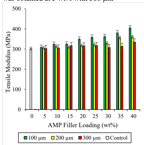
Figure 4: Effect of filler loading and particle size on tensile modulus of AMP/ER composites
