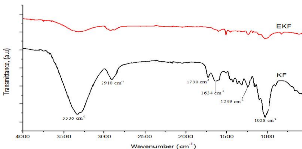
Figure 2b: The Combined spectra of raw kenaf (KF) and epoxy coated kenaf (EKF).
