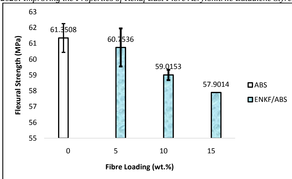
Figure 11: Flexural strength of kenaf fibre filled ABS composites at different fibre loadings
