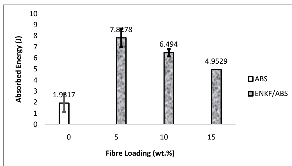
Figure 14: Impact absorbed energy of kenaf fibre filled ABS composites at different fibre loadings
