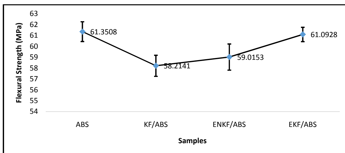
Figure 5: Chemical treatments effects on the flexural strength of kenaf fibre filled ABS composites at 10 wt% constant fibre loading.
