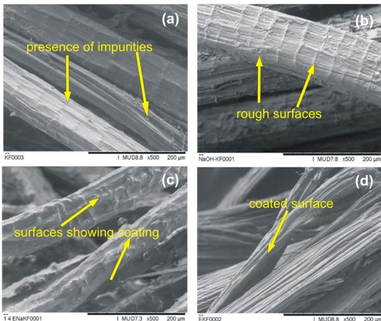
Figure 3: Morphology of (a) raw kenaf fibre (KF), (b) NaOH treated kenaf fibre (NKF), (c) epoxy coated-NaOH treated kenaf fibre (ENKF) and (d) epoxy coated kenaf fibre (EKF).
