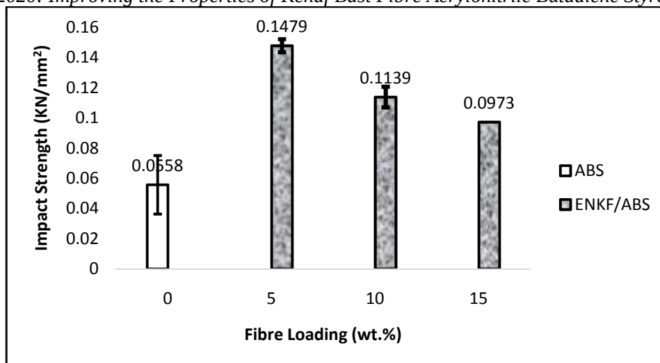
Figure 13: Impact strength of kenaf fibre filled ABS composites at different fibre loadings
