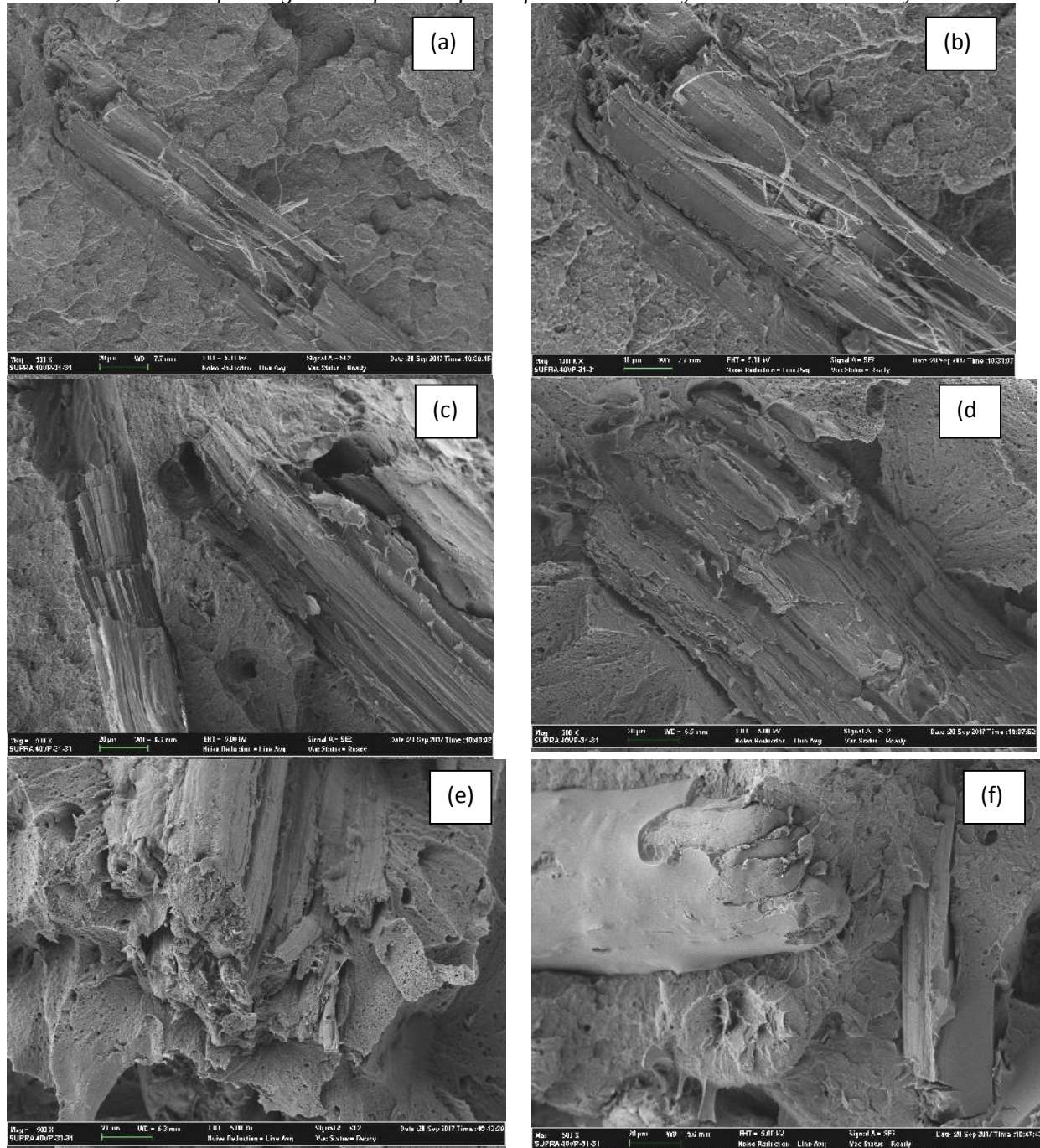
Figure 16: FESEM micrographs of epoxy-coated NaOH treated kenaf (ENKF/ABS) composites at 5 wt% (a, b), 10 wt% (c, d) and 15 wt% (e, f) fibre loadings.
