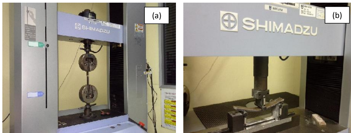
Figure 1: (a) Tensile testing procedure showing the test specimen clamped in the SHIMADZU Universal Tester and (b) Flexural testing procedure showing the 3-point bending configuration.
