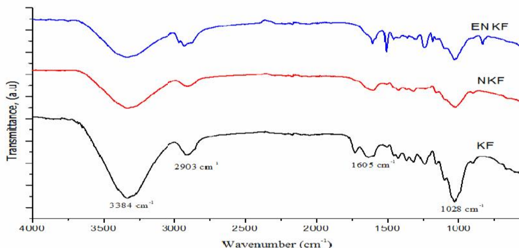
Figure 2a: The Spectra of raw kenaf (KF), NaOH-treated kenaf (NKF) and epoxy coated-treated kenaf (ENKF)
