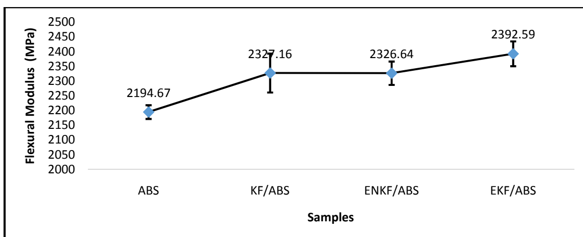
Figure 6: Chemical treatment effects on the flexural modulus of kenaf fibre filled ABS composites at 10 wt % constant fibre loading.
