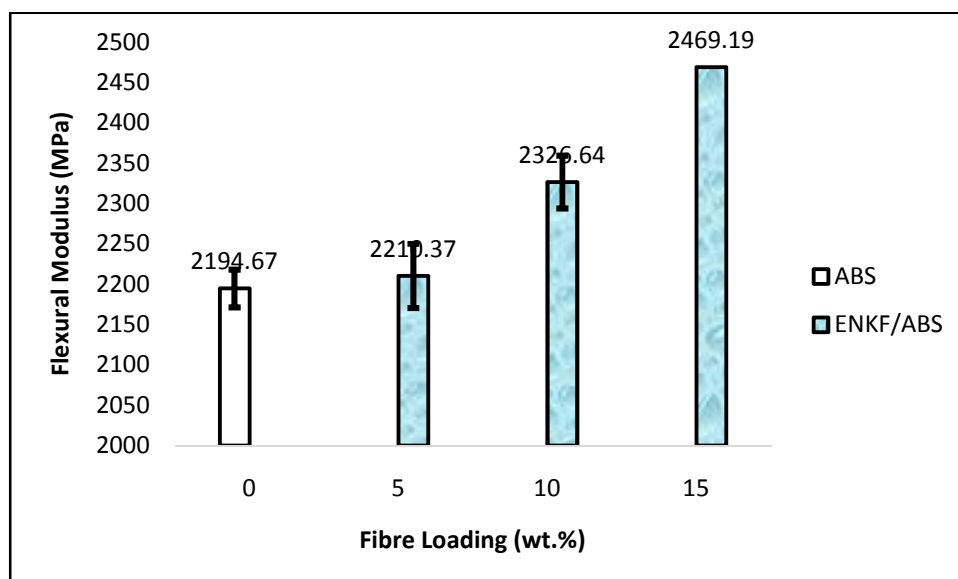
Figure 12: Flexural modulus of kenaf fibre filled ABS composites at different fibre loadings
