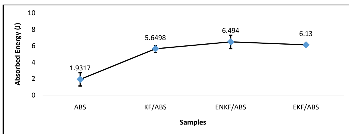
Figure 8: Chemical treatment effects on the impact absorbed energy of kenaf fibre filled ABS composites at 10 wt% constant fibre loading.
