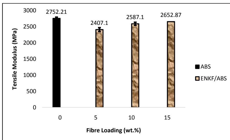
Figure 10: Tensile modulus of kenaf fibre filled ABS composites at different loadings
