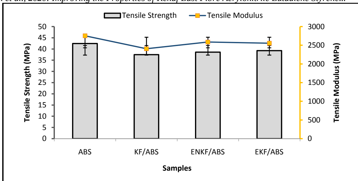
Figure 4: Several chemical treatments and their effect on the tensile strength and moduli of kenaf fibre filled ABS composites at 10 wt% constant fibre loading.
