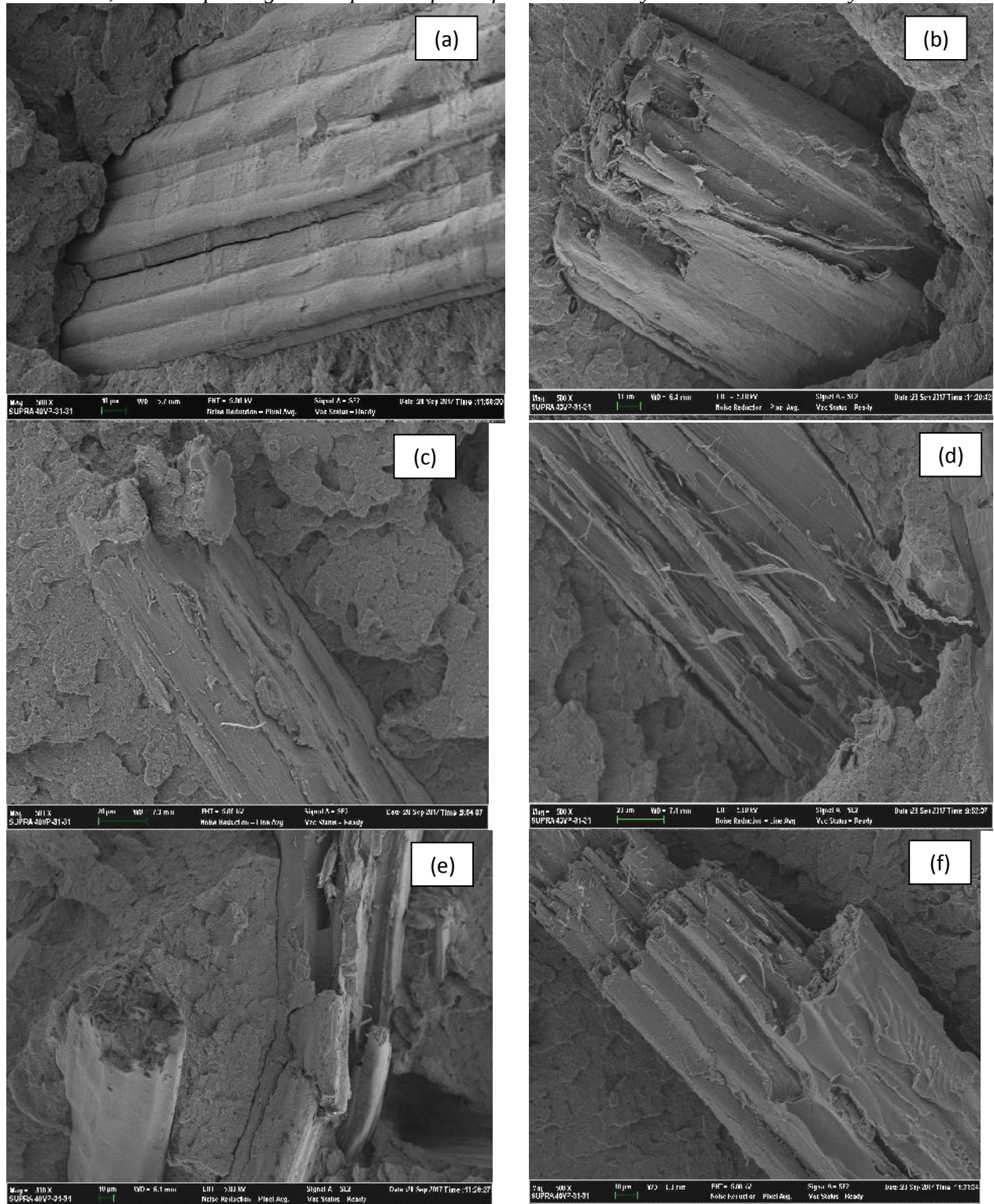
Figure 15: FESEM micrograph of raw kenaf, KF/ABS (a, b), epoxy-coated NaOH treated kenaf, ENKF/ABS (c, d) and epoxy-coated kenaf, EKF/ABS (e, f) composites.
