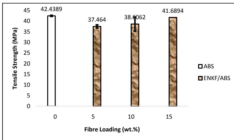
Figure 9: Effect of fibre loading on the tensile strength of kenaf fibre filled ABS composites
