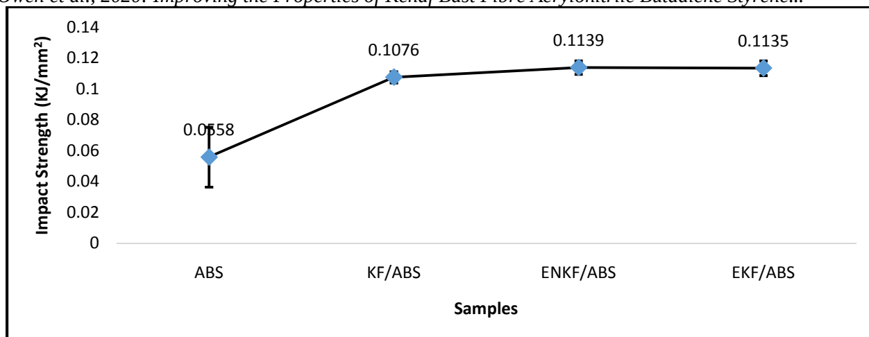
Figure 7: The chemical treatment effects on the impact strength of kenaf fibre filled ABS composites at 10 wt% constant fibre loading.
