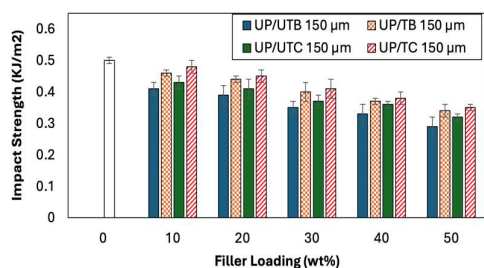
Figure 12: Effect of Filler Loading and Treatment on the Impact Strength of Polyester/Cowpea Husk and Polyester/Bambara nut shell Composites at 150 µm
