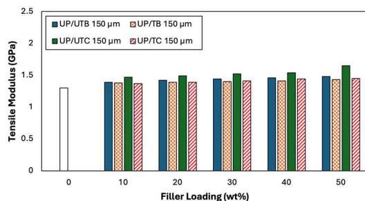
Figure 10: Effect of Filler Loading and Treatment on the Tensile Modulus of Polyester/Cowpea Husk and Polyester/Bambara nut shell Composites at 150 µm
