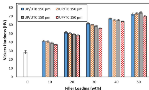
Figure 4: Effect of Filler Loading and treatment on the Hardness of Polyester/Cowpea Husk and Polyester/Bambara nut shell Composites at 150 µm
