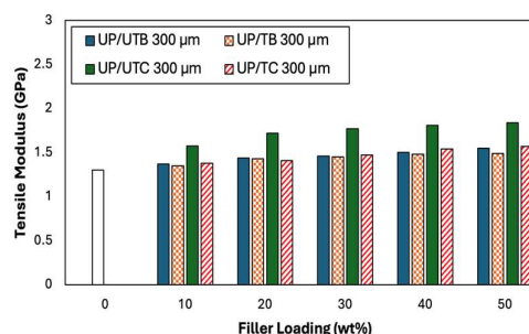
Figure 11: Effect of Filler Loading and Treatment on the Tensile Modulus of Polyester/Cowpea Husk and Polyester/Bambara nut shell Composites at 300 µm
