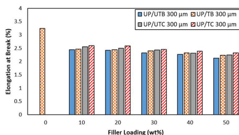
Figure 9: Effect of Filler Loading and Treatment on the Elongation at Break of Polyester/Cowpea Husk and Polyester/Bambara nut shell Composites at 300 µm
