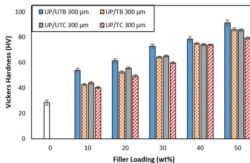
Figure 5: Effect of Filler Loading and Treatment on the Hardness of Polyester/Cowpea Husk and Polyester/Bambara nut shell Composites at 300 µm
