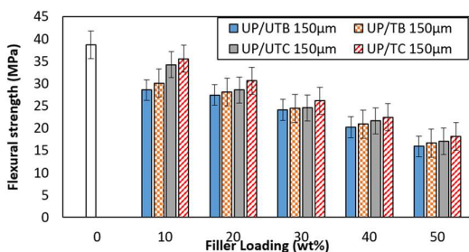
Figure 14: Effect of Filler Loading and treatment on the Flexural Strength of Polyester/Cowpea Husk and Polyester/Bambara nut shell Composites at 150 µm
