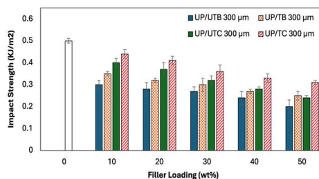
Figure 13: Effect of Filler Loading and Treatment on the Impact Strength of Polyester/Cowpea Husk and Polyester/Bambara nut shell Composites at 300 µm
