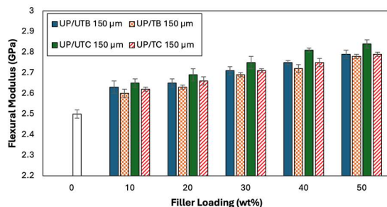
Figure 16: Effect of Filler Loading and Treatment on the Flexural Modulus of Polyester/Cowpea Husk and Polyester/Bambara nut shell Composites at 150 µm
