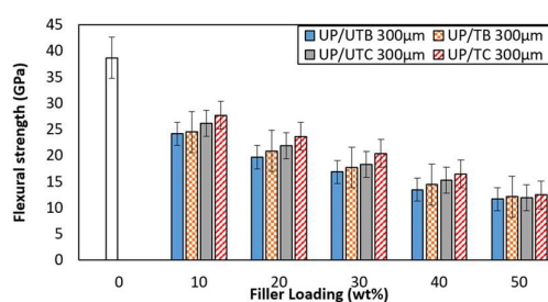
Figure 15: Effect of Filler Loading and Treatment on the Flexural Strength of Polyester/Cowpea Husk and Polyester/Bambara nut shell Composites at 300 µm
