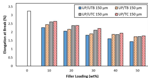
Figure 8: Effect of Filler Loading and Treatment on the Elongation at Break of Polyester/Cowpea Husk and Polyester/Bambara nut shell Composites at 150 µm
