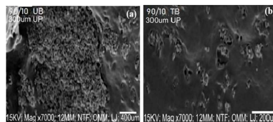
Figure 19: SEM Images for the Fractured Surfaces of (a) Untreated at 10 wt% (b) Treated at 10 wt% and Bambara nut Shell Composites of Polyester Resin at 300 µm
