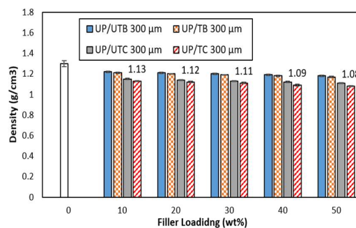
Figure 3: Effect of Filler Loading and Treatment on the Density of Polyester/Cowpea Husk and Polyester/Bambara nut shell Composites at 300 µm
