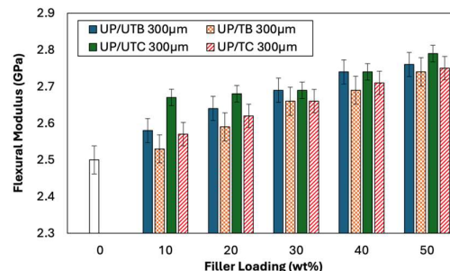
Figure 17: Effect of Filler Loading and Treatment on the Flexural Modulus of Polyester/Cowpea Husk and Polyester/Bambara nut shell Composites at 300 µm
