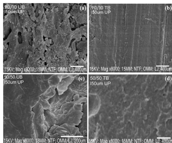
Figure 18: SEM Images for the Fractured Surfaces of (a) Untreated at 10 wt% (b) Treated at 10 wt% and (c) Untreated at 50 wt% (d) Treated at 50 wt% Bambara nut Shell Composites of Polyester Resin at 150 µm
