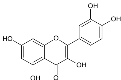
Figure 1: Structure of the colouring pigment (Quercetin) in onion outer scale.
