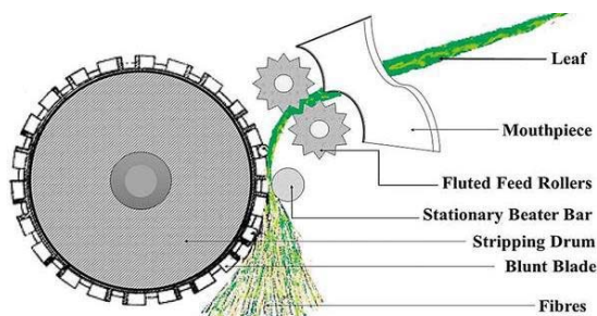
Fig. 3: Pseudo-stem fibre extraction machine.
