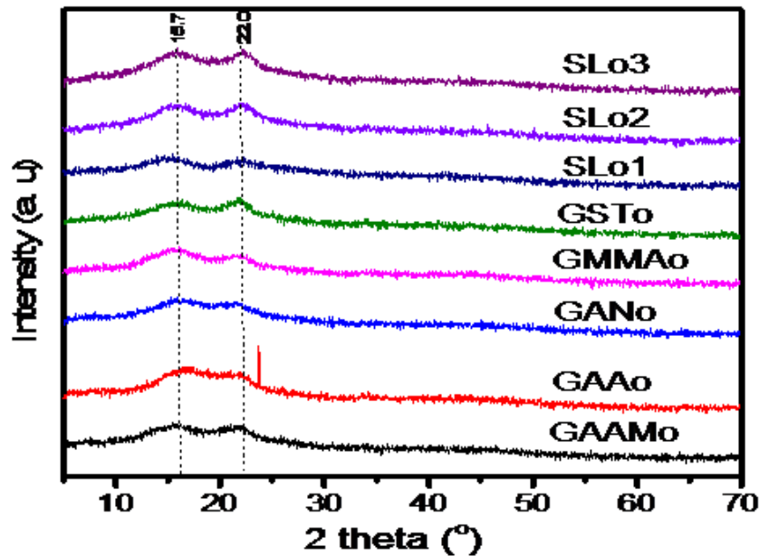
Figure 4.1 X-ray Diffractogram
