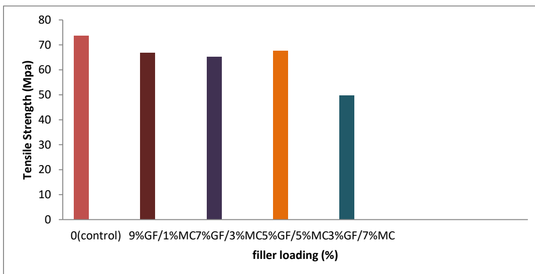
Figure 1: Tensile Strength against Filler loading of GF/MC/ER Hybrid Composites.
