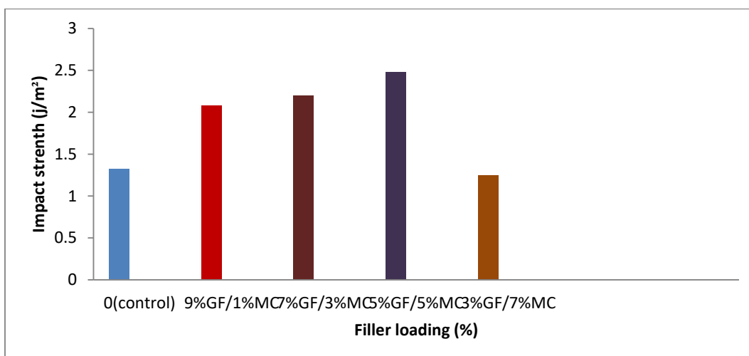
Figure 3: Impact Strength Against Filler Loading of GF/MC/ER Hybrid Composites.
