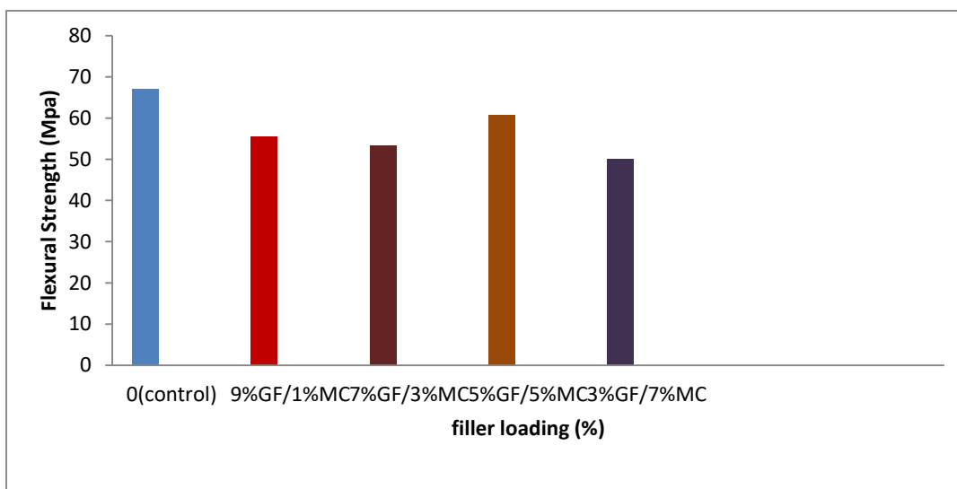
Figure 2: Flexural strength against Filler loading of GF/MC/ER Hybrid Composites
