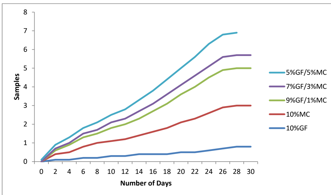
Figure 5: Water Absorption against the number of days for GF/ MC/ER composites
