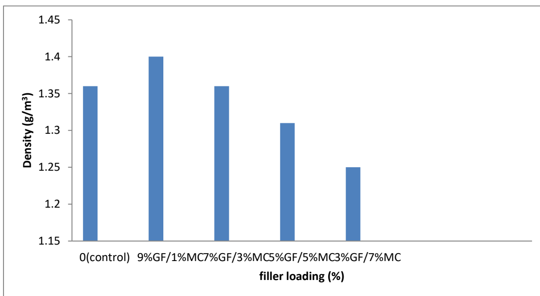
Figure 4: Density against Filler Content of GF/MC/ER Hybrid Composites
