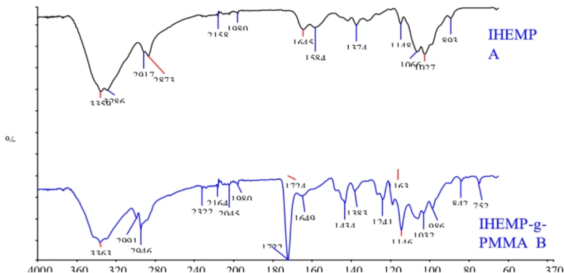
Figure 2: FTIR spectra of (a) ungrafted Ihemp preform and (b) Ihemp-g-PMMA.
