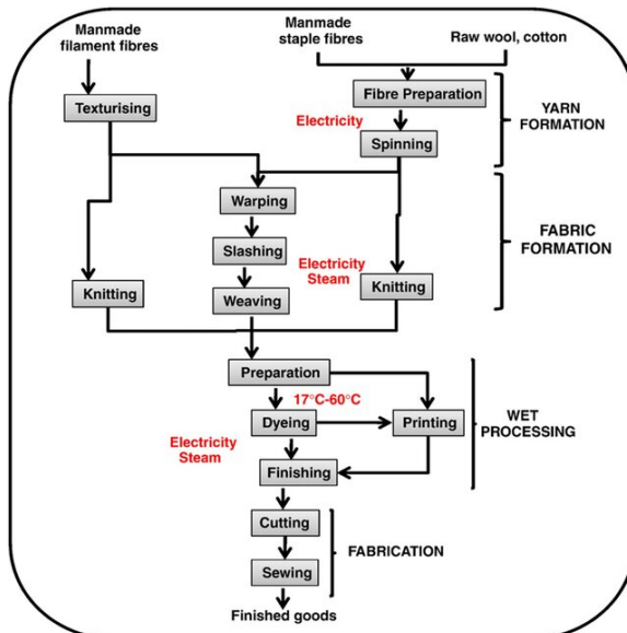
Fig. 4: Processing flow of textile products with energy indication. Source: Martínez (2010)
